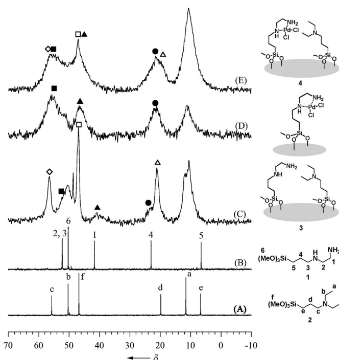
Figure 2. Liquid-state 13 C NMR spectra of A) 3-diethylaminopropyl-trimethoxysilane ( 2 ), and B) 3-(2-aminoethylamino)propyl-trimethoxysilane ( 1 ), and solid-state 13 C CP/MAS NMR spectra of C) SiO 2 /diamine/NEt 3 ( 3 ), D) SiO 2 /diamine/Pd, and E) SiO 2 /diamine/Pd/NEt 3 ( 4 ). Definitions of symbols; ▲ and ■: carbon atoms connected to nitrogen atoms of the diamine functional group, ●: central carbon atom in the propyl chain of the diamine functional group, Δ and ◇: carbon atoms of the tertiary amine functional group, □: methoxy groups.
