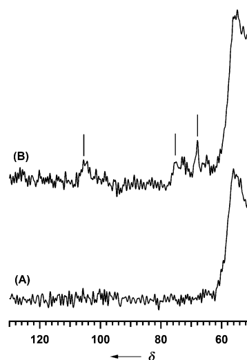
Figure 3. Solid-state 13 C CP/MAS NMR spectra of A) SiO 2 /diamine/Pd/NEt 3 ( 4 ) and B) SiO 2 /diamine/Pd/NEt 3 ( 4 ) treated with allylmethylcarbonate. Signals at around 70 and at 106 ppm correspond to terminal and center carbon atoms, respectively, of the \eta^3 -allylpalladium species. [10]
